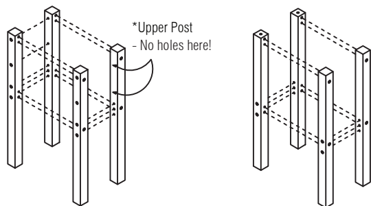
(A) Upper Post (Short) x 4 (B) Upper Post (Long) x 4
