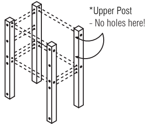
(A) Upper Post (Shorter) x 4
